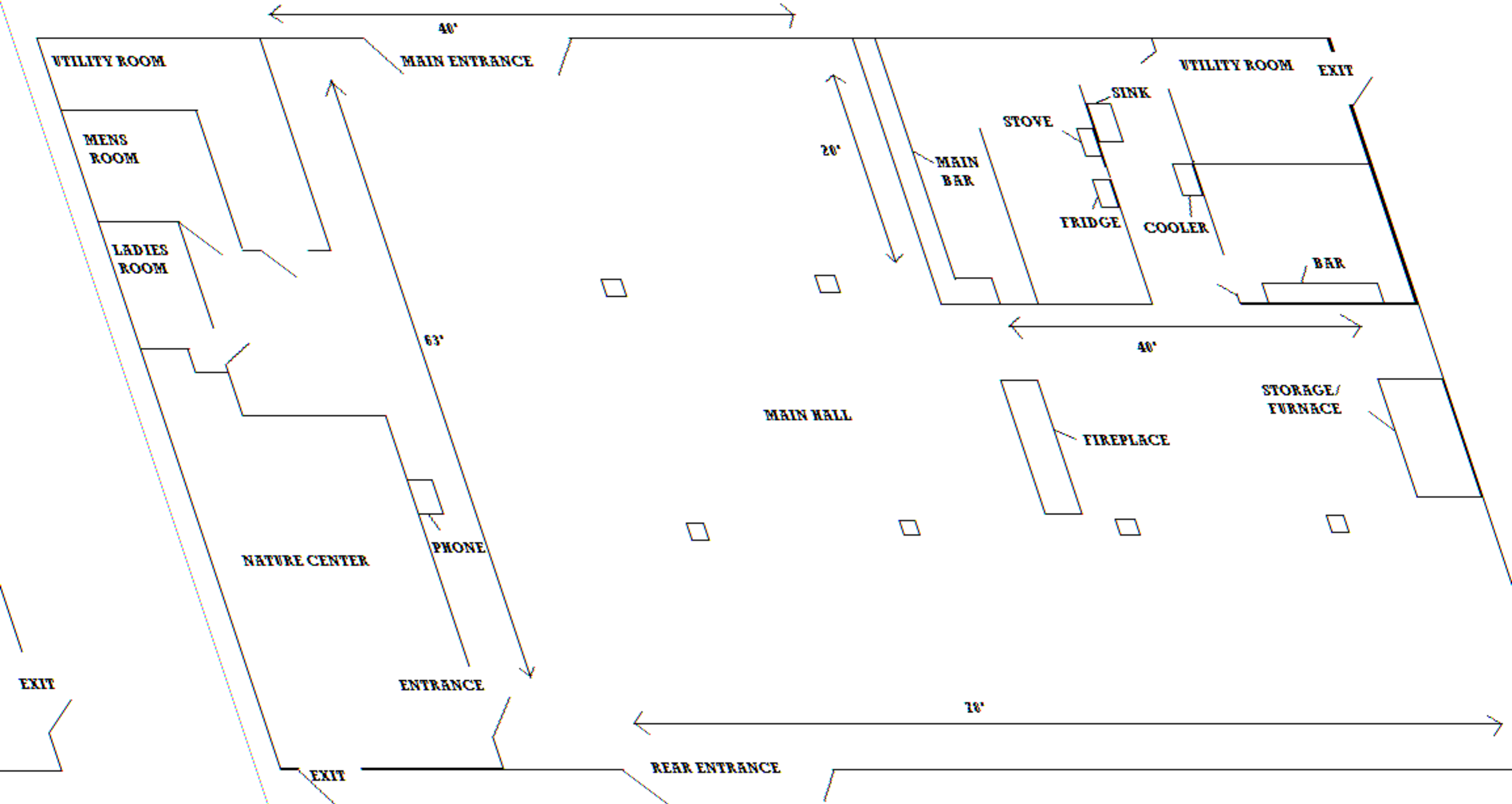
BOND LAKE WARMING HOUSE FLOOR PLAN
